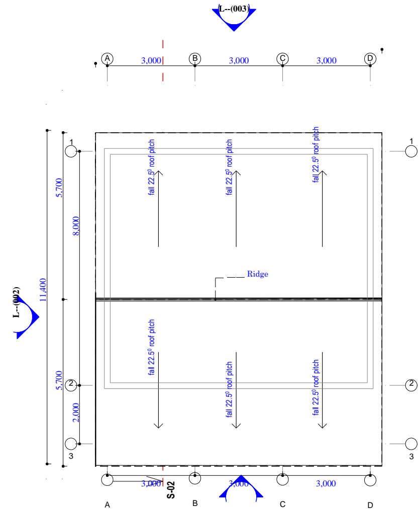
ROOF PLAN
